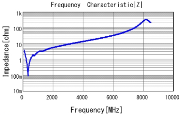
■ GRM1885C2A391JA01 |Z| DCOV, 25degC
