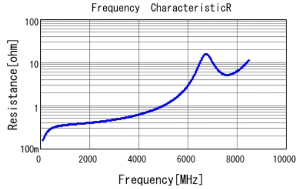
■ GRM1885C2A4R7CA01 R DCOV, 25degC
