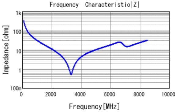
■ GRM1885C2A4R7CA01 |Z| DCOV, 25degC
