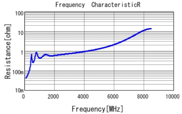
■ GRM1885C2A821JA01 R DCOV, 25degC
