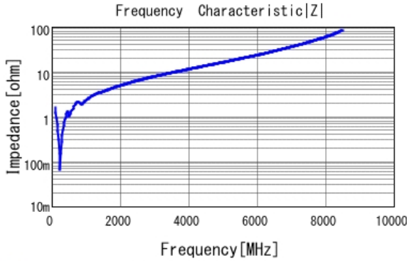
■ GRM1885C2A821JA01 |Z| DCOV, 25degC
