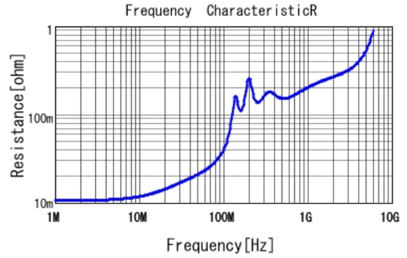
■ GRM1887U1H103JA01 R DCOV, 25degC
