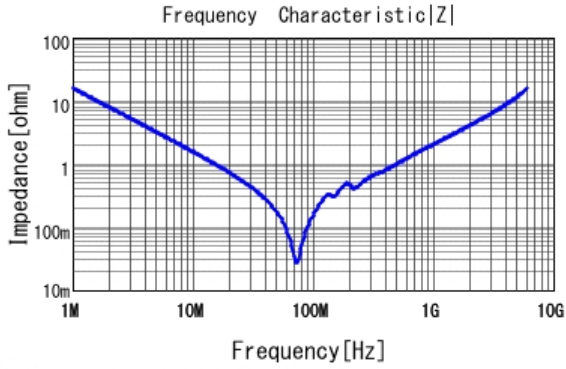
■ GRM1887U1H103JA01 |Z| DCOV, 25degC
