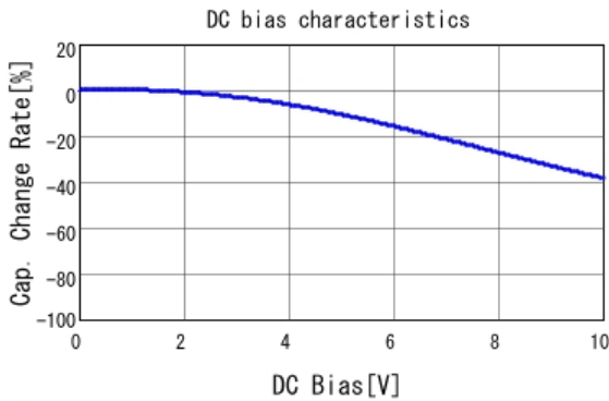
■ GRM188B11A105KA61 C-DC bias capchange, 20.0degC, AC1.
