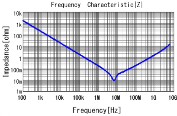
■ GRM188B11A105KA61 |Z| DCOV, 20degC
