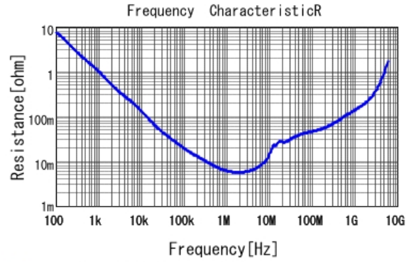
■ GRM188B11A105KA61 R DCOV, 20degC
