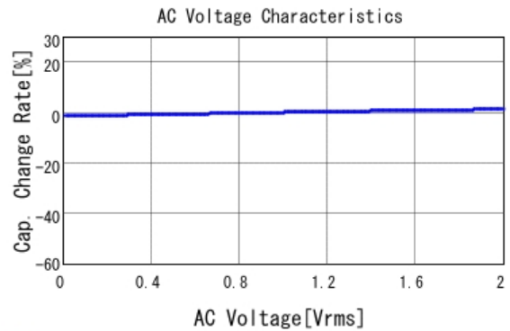
■ GRM188B11H221KA01 C-AC Voltage capchange, DCOV, 20.0d
