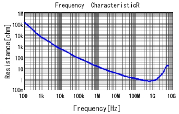
■ GRM188B11H221KA01 R DCOV, 20degC
