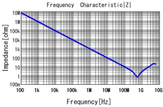
■ GRM188B11H221KA01 |Z| DCOV, 20degC
