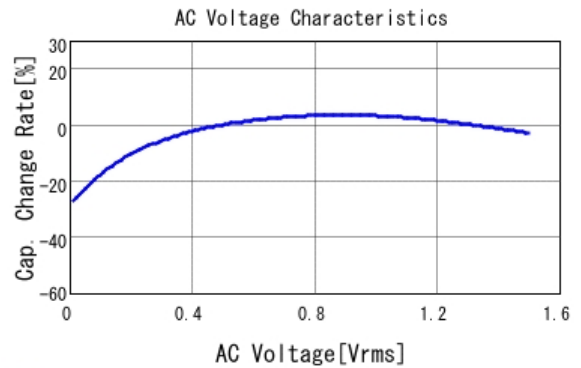
■ GRM188B30J226MEA0 C-AC Voltage capchange, DCOV, 20.0d
