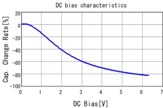
■ GRM188B30J226MEA0 C-DC bias capchange, 20.0degC, AC0.
