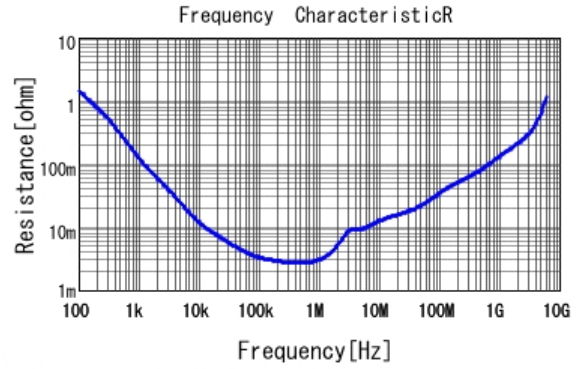
■ GRM188B30J226MEA0 R DCOV, 20degC
