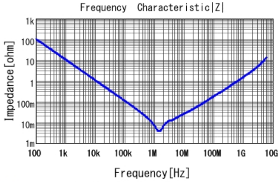
■ GRM188B30J226MEA0 |Z| DCOV, 20degC
