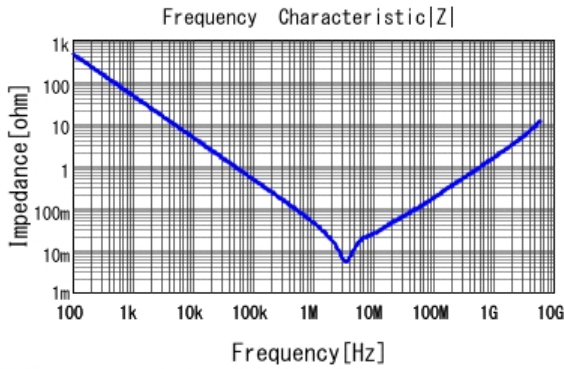
■ GRM188B30J475KE18 |Z| DCOV, 20degC
