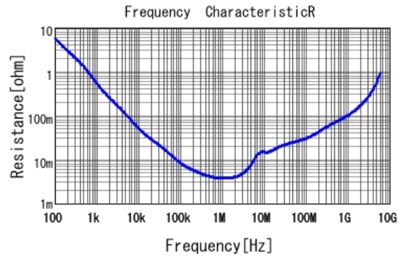
■ GRM188B30J475KE18 R DCOV, 20degC
