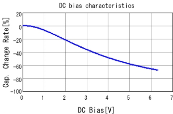
■ GRM188B30J475KE18 C-DC bias capchange, 20.0degC, AC0.
