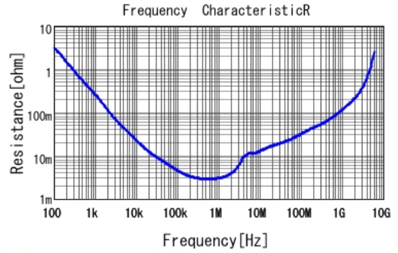
■ GRM188B31A106ME69 R DCOV, 20degC
