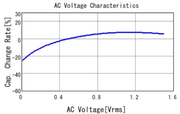
■ GRM188B31A106ME69 C-AC Voltage capchange, DCOV, 20.0d
