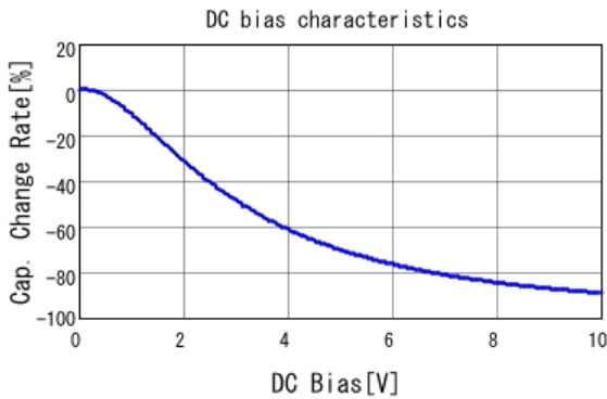
■ GRM188B31A106ME69 C-DC bias capchange, 20.0degC, AC0.
