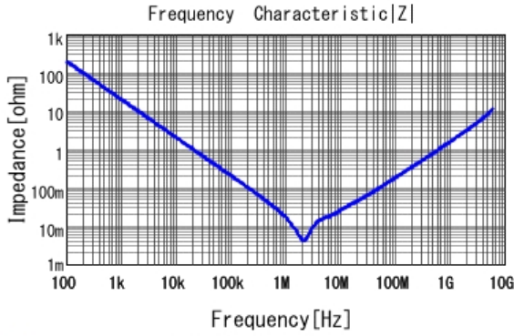
■ GRM188B31A106ME69 |Z| DCOV, 20degC
