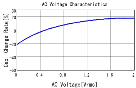
■ GRM188B31A225KE33 C-AC Voltage capchange, DCOV, 20.0d
