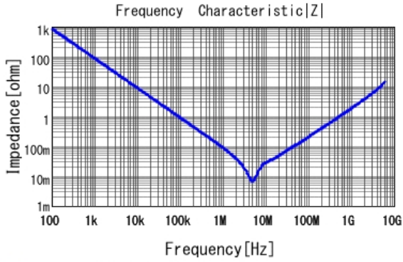
■ GRM188B31A225KE33 |Z| DCOV, 20degC
