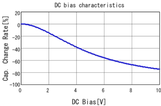
■ GRM188B31A225KE33 C-DC bias capchange, 20.0degC, AC0.
