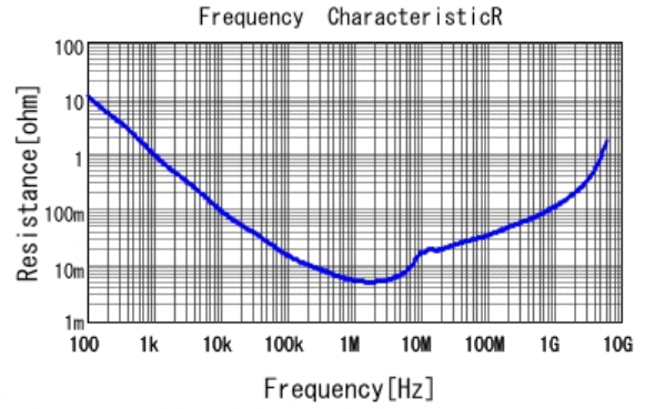
■ GRM188B31A225KE33 R DCOV, 20degC
