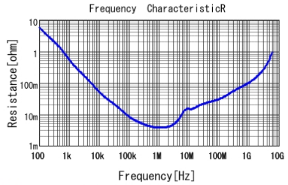
■ GRM188B31A475KE15 R DCOV, 20degC
