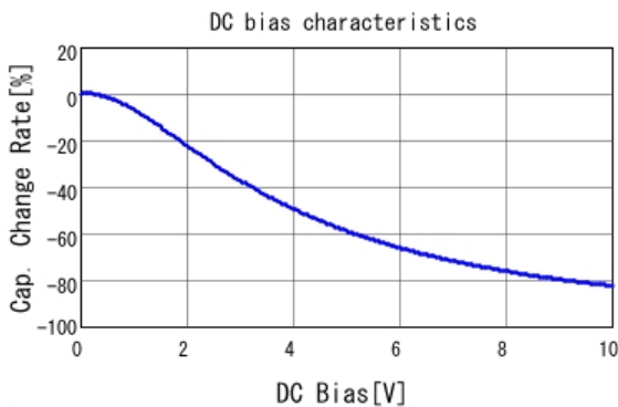
■ GRM188B31A475KE15 C-DC bias capchange, 20.0degC, AC0.
