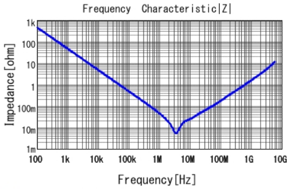
■ GRM188B31A475KE15 |Z| DCOV, 20degC
