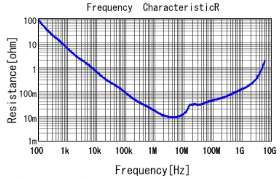
■ GRM188B31C105KA92 R DCOV, 20degC
