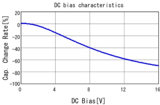
■ GRM188B31C105KA92 C-DC bias capchange, 20.0degC, AC1.
