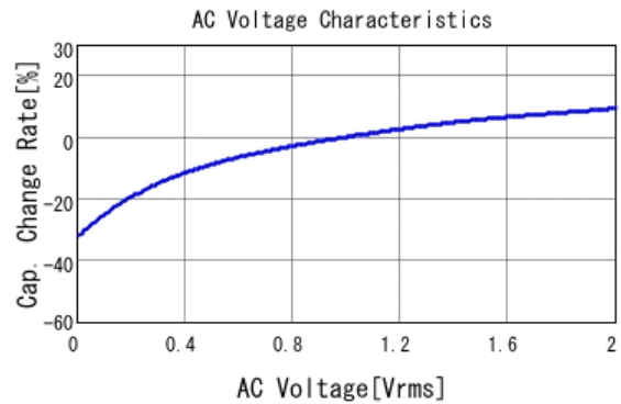
■ GRM188B31C105KA92 C-AC Voltage capchange, DCOV, 20.0d
