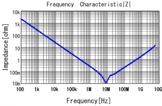
■ GRM188B31C105KA92 |Z| DCOV, 20degC
