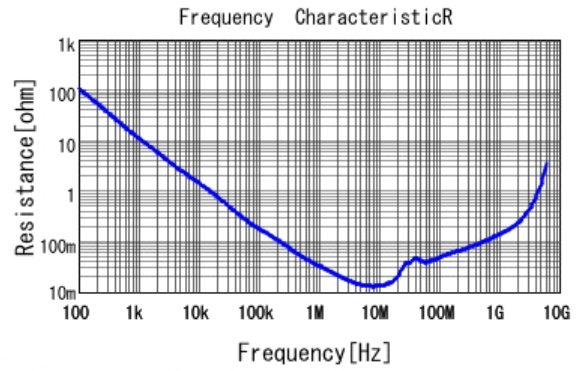
■ GRM188B31E474KA75 R DCOV, 20degC
