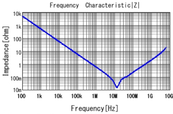
■ GRM188B31E474KA75 |Z| DCOV, 20degC
