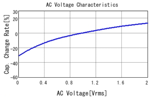
■ GRM188B31E474KA75 C-AC Voltage capchange, DCOV, 20.0d
