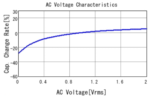
■ GRM188C71A475KE11 C-AC Voltage capchange, DCOV, 25.0d
