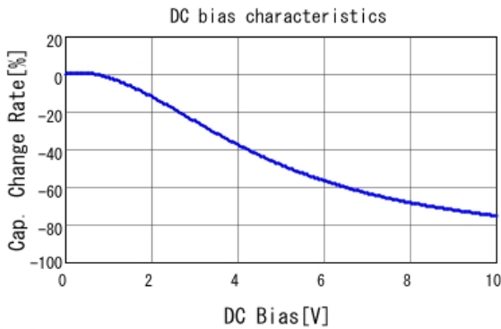
■ GRM188C71A475KE11 C-DC bias capchange, 25.0degC, AC1V
