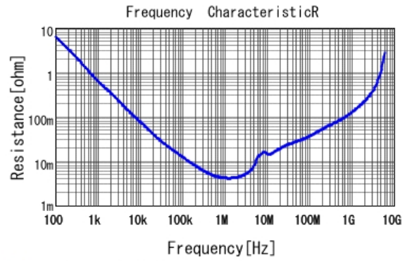
■ GRM188C71A475KE11 R DCOV, 25degC
