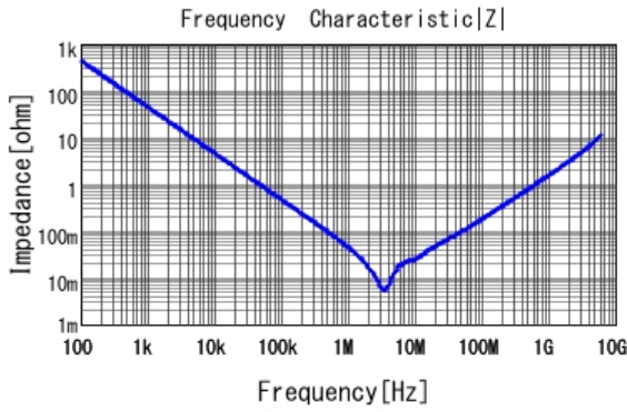
■ GRM188C71A475KE11 |Z| DCOV, 25degC
