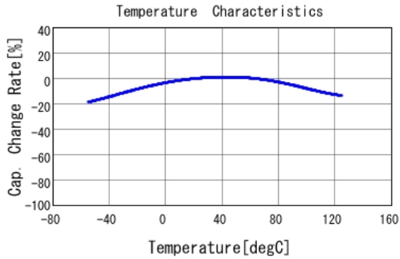
■ GRM188C71C225KE11 C-Temp. capchange, DCO. 0V, ACO. 2Vrm
