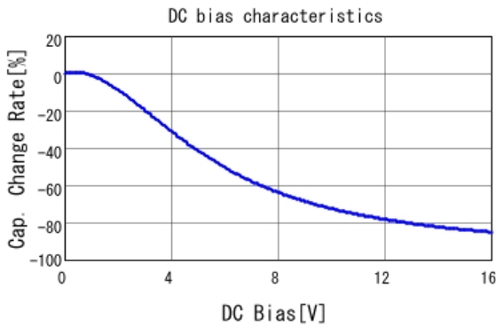
■ GRM188C71C475ME21 C-DC bias capchange, 25.0degC, AC1V
