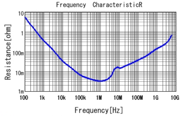
■ GRM188C71C475ME21 R DCOV, 25degC
