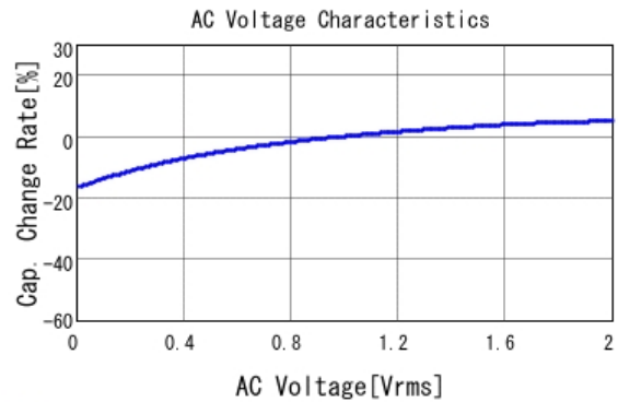
■ GRM188C71C475ME21 C-AC Voltage capchange, DCOV, 25.0d
