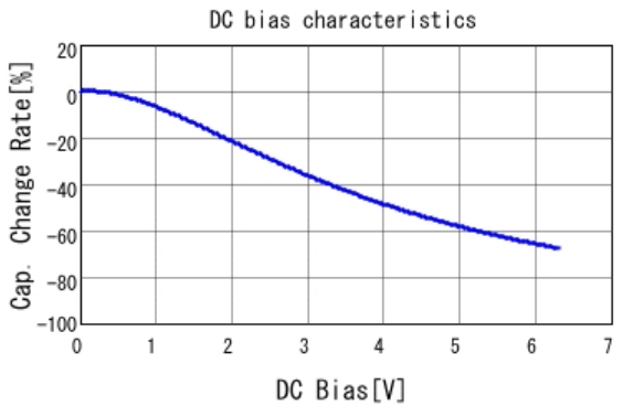
■ GRM188C80J475KE15 C-DC bias capchange, 25.0degC, AC0.
