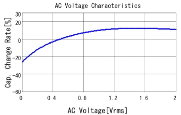
■ GRM188C80J475KE15 C-AC Voltage capchange, DCOV, 25.0d
