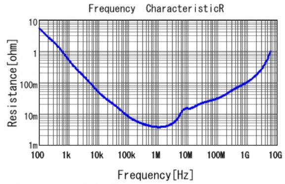
■ GRM188C80J475KE15 R DCOV, 25degC
