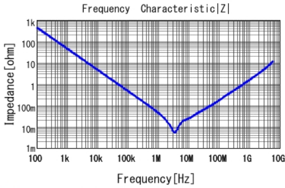
■ GRM188C80J475KE15 |Z| DCOV, 25degC
