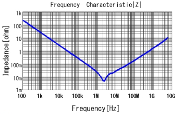
■ GRM188C81C106MA73 |Z| DCOV, 25degC
