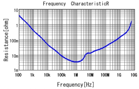
■ GRM188C81C106MA73 R DCOV, 25degC
