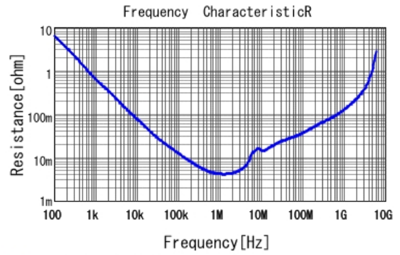
■ GRM188C81C475KE11 R DCOV, 25degC
