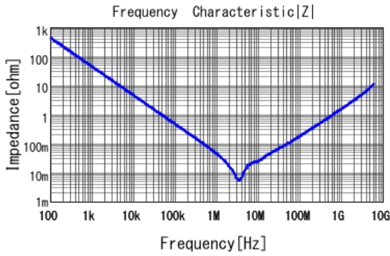
■ GRM188C81C475KE11 |Z| DCOV, 25degC
