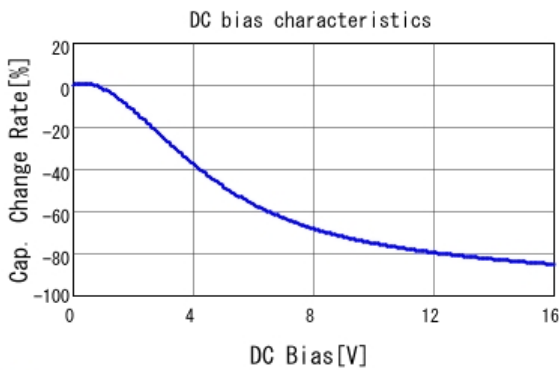
■ GRM188C81C475KE11 C-DC bias capchange, 25.0degC, AC1V
