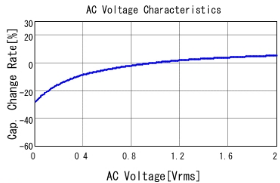
■ GRM188C81C475KE11 C-AC Voltage capchange, DCOV, 25.0d
