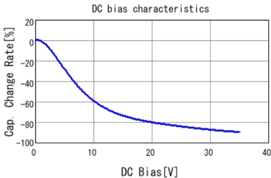
■ GRM188C8YA225KE11 C-DC bias capchange, 25.0degC, AC1V
