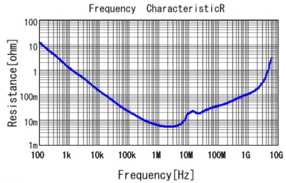
■ GRM188C8YA225KE11 R DCOV, 25degC
