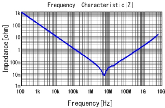
■ GRM188C8YA225KE11 |Z| DCOV, 25degC
