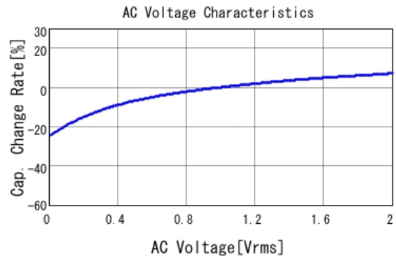
■ GRM188C8YA225KE11 C-AC Voltage capchange, DCOV, 25.0d
