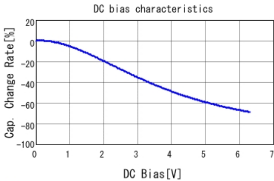
■ GRM188D70J106MA73 C-DC bias capchange, 25.0degC, AC1V
