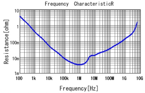
■ GRM188D70J106MA73 R DCOV, 25degC
