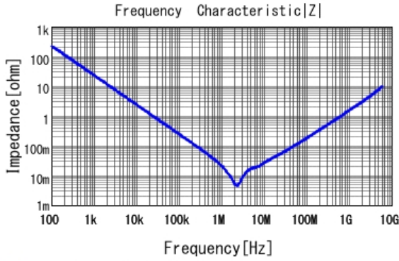
■ GRM188D70J106MA73 |Z| DCOV, 25degC
