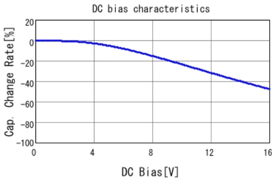
■ GRM188R11C474KA88 C-DC bias capchange, 20.0degC, AC1.
