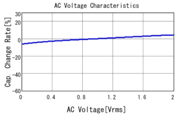
■ GRM188R11C474KA88 C-AC Voltage capchange, DCOV, 20.0d
