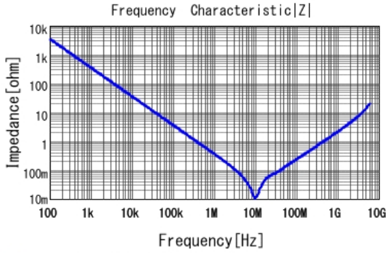
■ GRM188R11C474KA88 |Z| DCOV, 20degC
