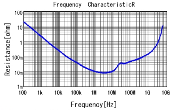
■ GRM188R11C474KA88 R DCOV, 20degC
