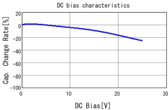
■ GRM188R11E333KA01 C-DC bias capchange, 20.0degC, AC1.
