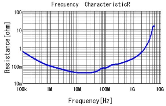
■ GRM188R11E333KA01 R DCOV, 20degC
