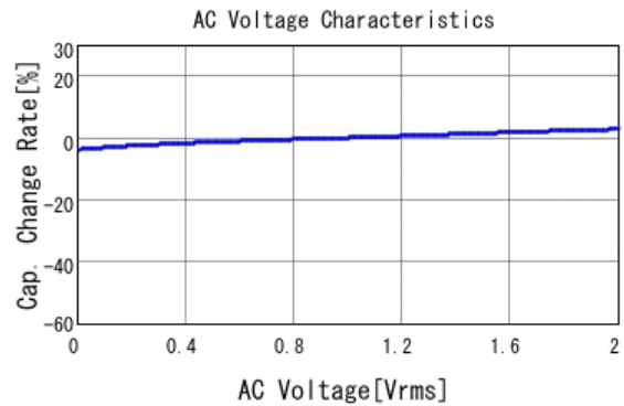
■ GRM188R11E333KA01 C-AC Voltage capchange, DCOV, 20.0d
