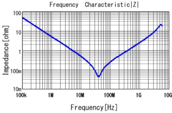
■ GRM188R11E333KA01 |Z| DCOV, 20degC
