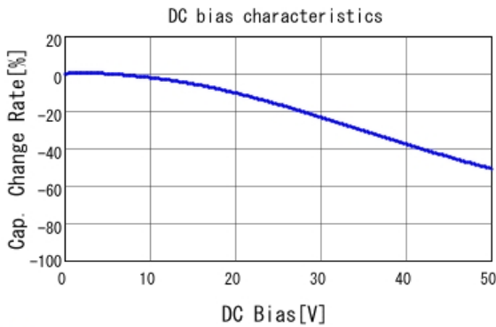
■ GRM188R11H104KA93 C-DC bias capchange, 20.0degC, AC1.
