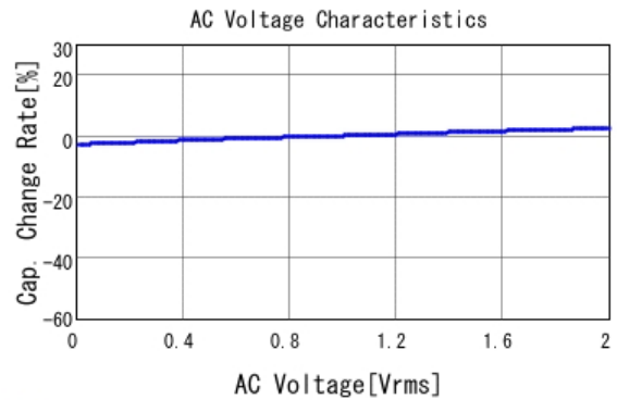
■ GRM188R11H104KA93 C-AC Voltage capchange, DCOV, 20.0d
