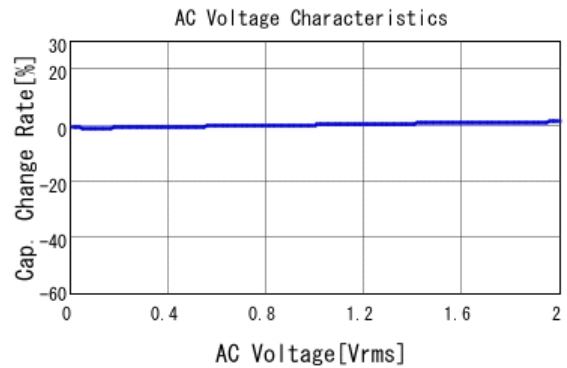
■ GRM188R11H471KA01 C-AC Voltage capchange, DCOV, 20.0d
