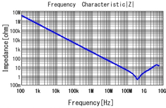
■ GRM188R11H471KA01 |Z| DCOV, 20degC
