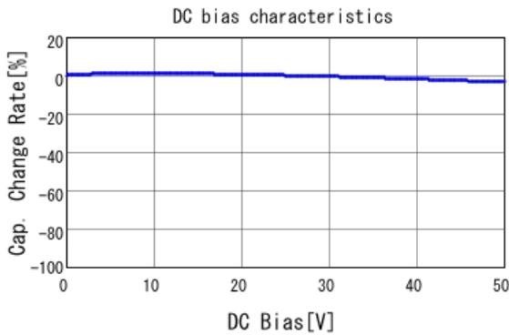
■ GRM188R11H471KA01 C-DC bias capchange, 20.0degC, AC1.
