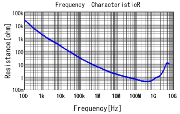
■ GRM188R11H471KA01 R DCOV, 20degC
