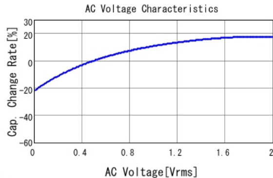
■ GRM188R60J225KE19 C-AC Voltage capchange, DCOV, 25.0d
