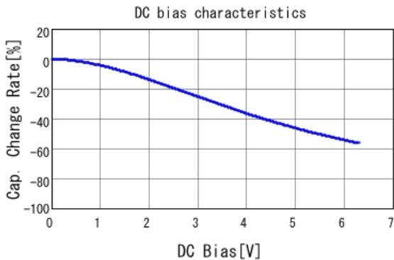
■ GRM188R60J225KE19 C-DC bias capchange, 25.0degC, ACO.
