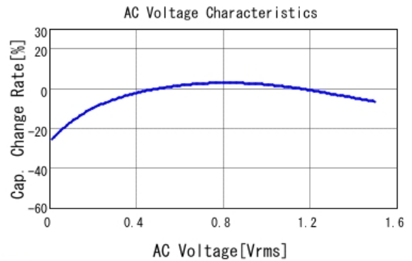
■ GRM188R60J226MEA0 C-AC Voltage capchange, DCOV, 25.0d
