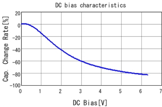
■ GRM188R60J226MEA0 C-DC bias capchange, 25.0degC, AC0.
