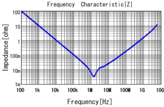
■ GRM188R60J226MEA0 |Z| DCOV, 25degC
