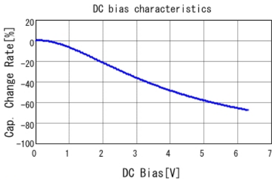
■ GRM188R60J475KE19 C-DC bias capchange, 25.0degC, AC0.
