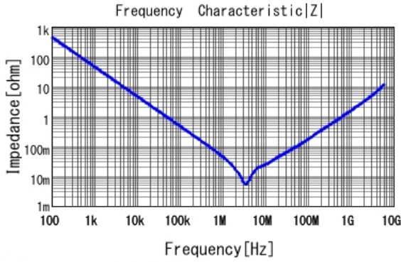
■ GRM188R60J475KE19 |Z| DCOV, 25degC
