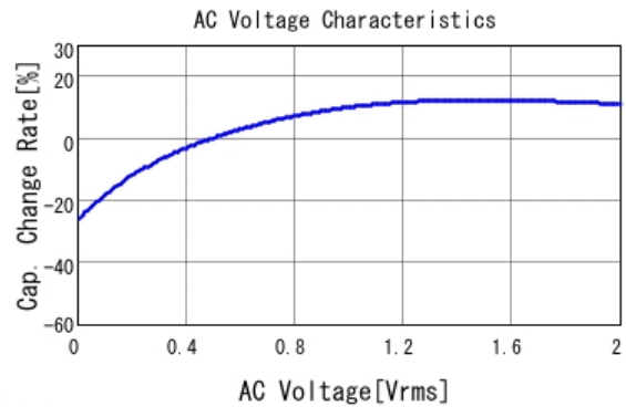
■ GRM188R60J475KE19 C-AC Voltage capchange, DCOV, 25.0d
