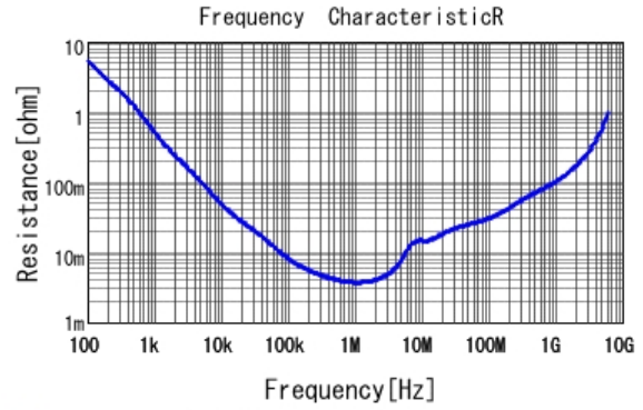
■ GRM188R60J475KE19 R DCOV, 25degC
