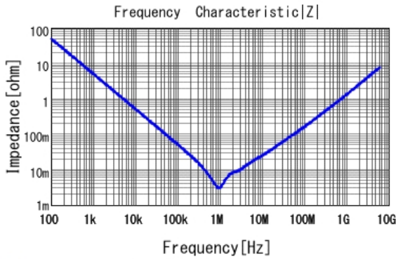
■ GRM188R60J476ME15 |Z| DCOV, 25degC
