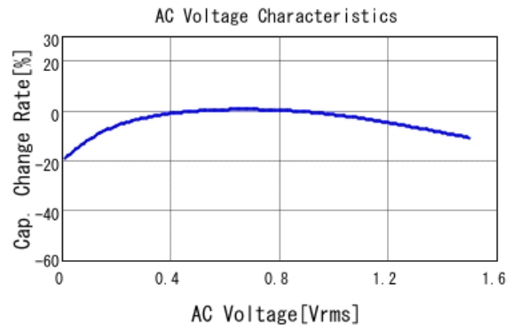
■ GRM188R60J476ME15 C-AC Voltage capchange, DCOV, 25.0d
