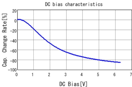
■ GRM188R60J476ME15 C-DC bias capchange, 25.0degC, ACO.
