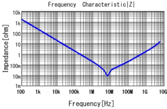
■ GRM188R61A105KA61 |Z| DCOV, 25degC
