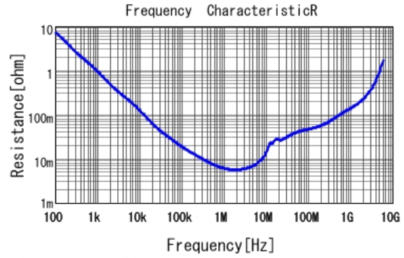
■ GRM188R61A105KA61 R DCOV, 25degC
