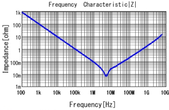
■ GRM188R61A225KE34 |Z| DCOV, 25degC
