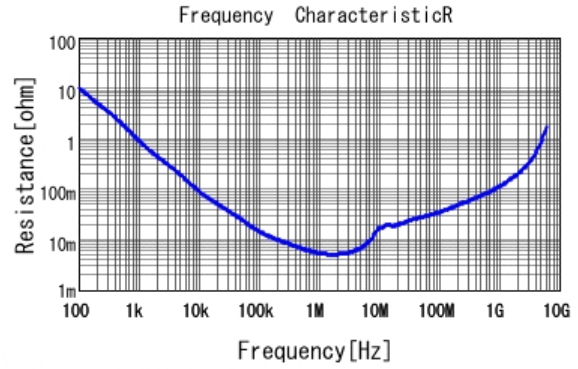
■ GRM188R61A225KE34 R DCOV, 25degC
