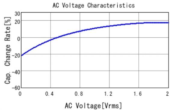
■ GRM188R61A225KE34 C-AC Voltage capchange, DCOV, 25.0d
