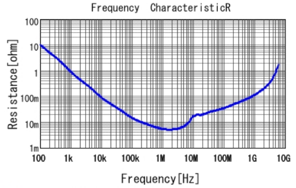
■ GRM188R61A225ME34 R DCOV, 25degC
