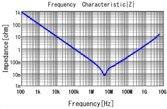
■ GRM188R61A225ME34 |Z| DCOV, 25degC
