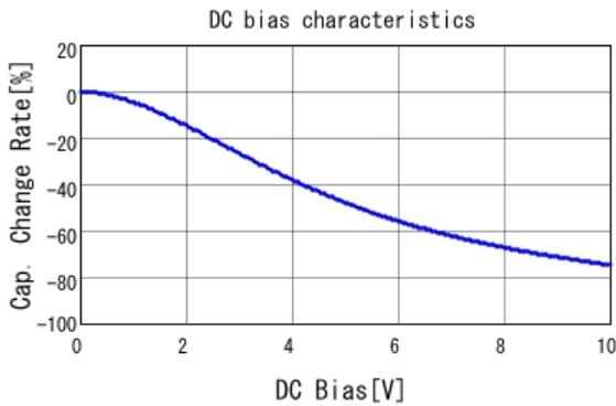
■ GRM188R61A225ME34 C-DC bias capchange, 25.0degC, AC0.
