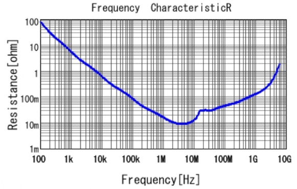
■ GRM188R61C105KA93 R DCOV, 25degC
