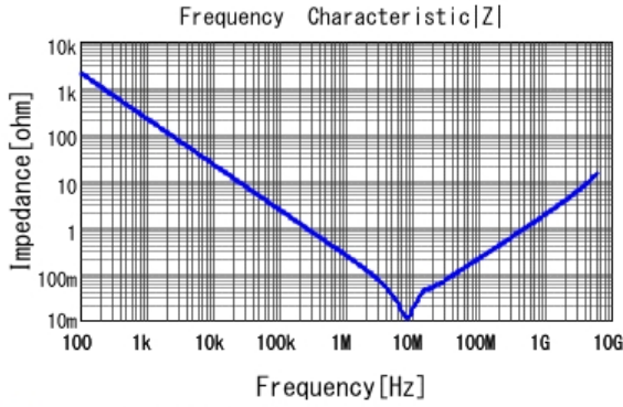
■ GRM188R61C105KA93 |Z| DCOV, 25degC
