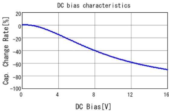
■ GRM188R61C105KA93 C-DC bias capchange, 25.0degC, AC1.
