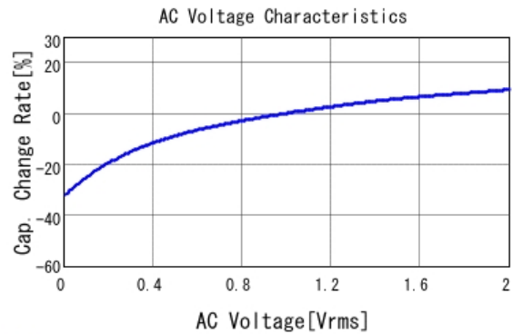
■ GRM188R61C105KA93 C-AC Voltage capchange, DCOV, 25.0d
