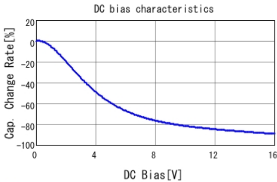
■ GRM188R61C106MA73 C-DC bias capchange, 25.0degC, AC1V
