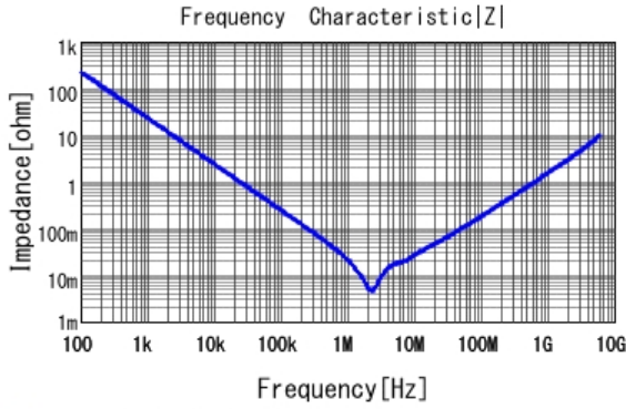
■ GRM188R61C106MA73 |Z| DCOV, 25degC
