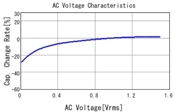
■ GRM188R61C106MA73 C-AC Voltage capchange, DCOV, 25.0d
