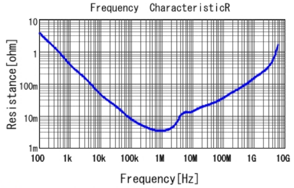
■ GRM188R61C106MA73 R DCOV, 25degC
