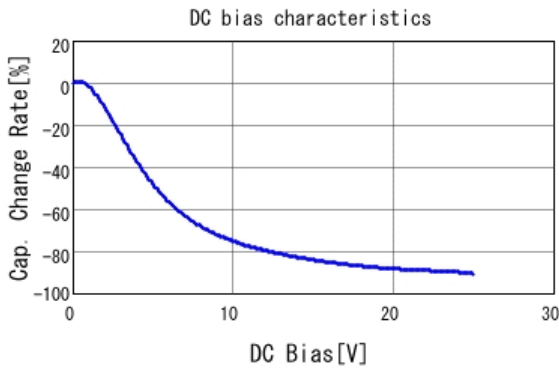
■ GRM188R61E475KE11 C-DC bias capchange, 25.0degC, AC1V
