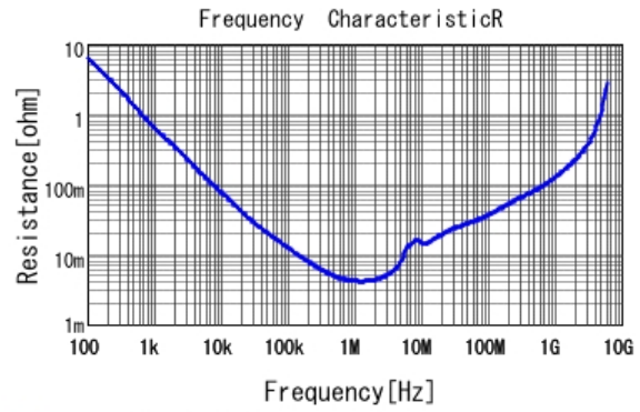
■ GRM188R61E475KE11 R DCOV, 25degC
