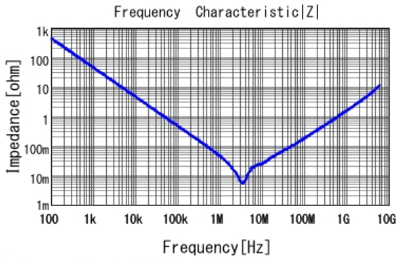
■ GRM188R61E475KE11 |Z| DCOV, 25degC
