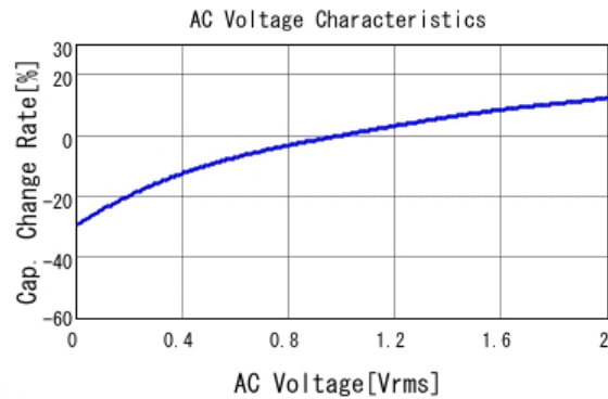
■ GRM188R61H474MA12 C-AC Voltage capchange, DCOV, 25.0d
