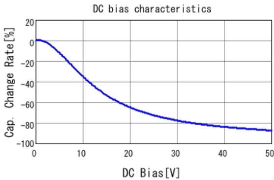
■ GRM188R61H474MA12 C-DC bias capchange, 25.0degC, AC1V
