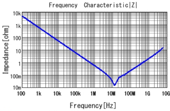
■ GRM188R61H474MA12 |Z| DCOV, 25degC
