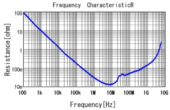
■ GRM188R61H474MA12 R DCOV, 25degC
