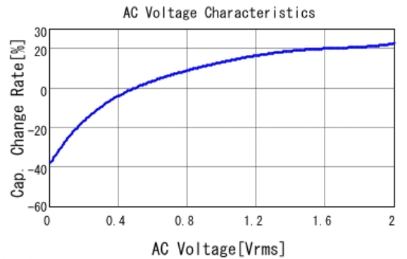
■ GRM188R70J225KE15 C-AC Voltage capchange, DCOV, 25.0d
