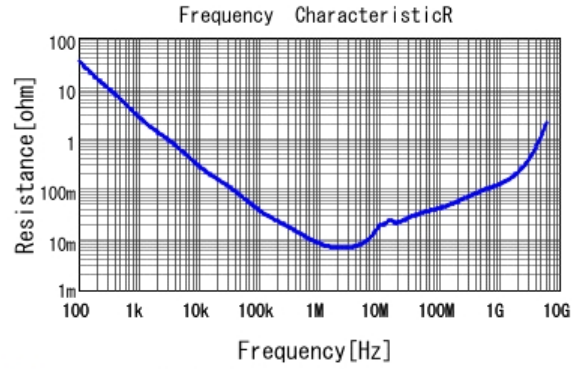
■ GRM188R70J225KE15 R DCOV, 25degC
