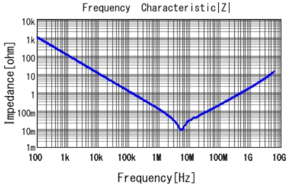
■ GRM188R70J225KE15 |Z| DCOV, 25degC
