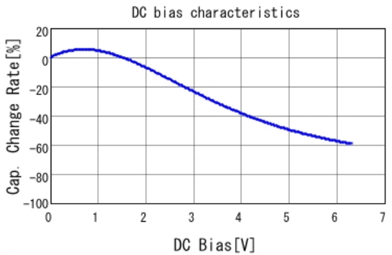
■ GRM188R70J225KE15 C-DC bias capchange, 25.0degC, AC0.
