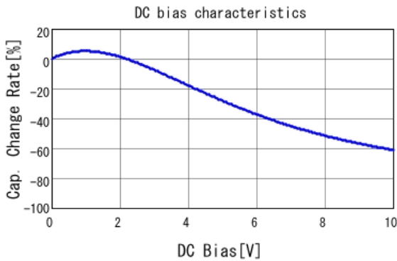
■ GRM188R71A105KA61 C-DC bias capchange, 25.0degC, AC1.
