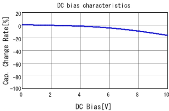
■ GRM188R71A154KA01 C-DC bias capchange, 25.0degC, AC1.
