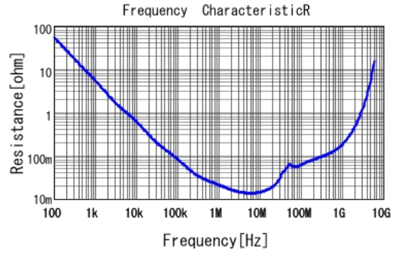
■ GRM188R71A154KA01 R DCOV, 25degC
