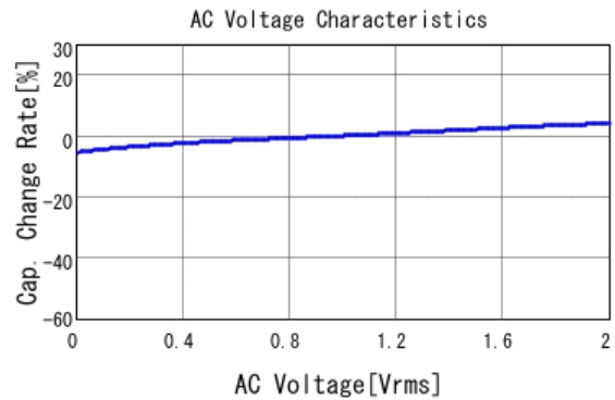
■ GRM188R71A154KA01 C-AC Voltage capchange, DCOV, 25.0d
