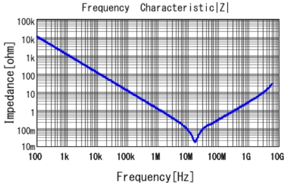
■ GRM188R71A154KA01 |Z| DCOV, 25degC
