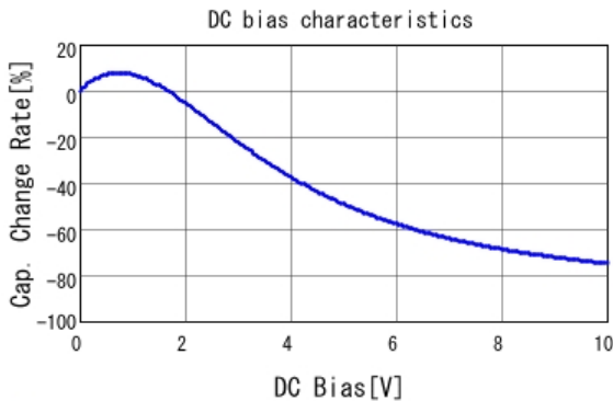
■ GRM188R71A225KE15 C-DC bias capchange, 25.0degC, AC0.
