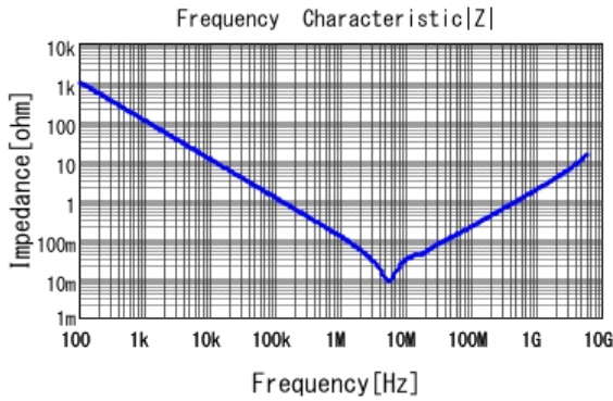
■ GRM188R71A225KE15 |Z| DCOV, 25degC
