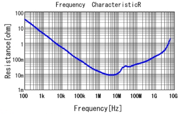
■ GRM188R71C105KE15 R DCOV, 25degC
