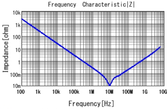
■ GRM188R71C105KE15 |Z| DCOV, 25degC
