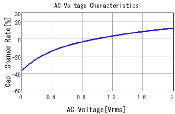
■ GRM188R71C105KE15 C-AC Voltage capchange, DCOV, 25.0d
