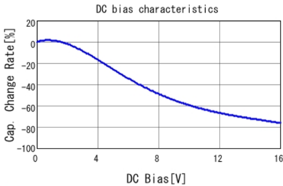
■ GRM188R71C105KE15 C-DC bias capchange, 25.0degC, AC1V
