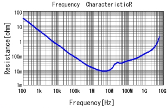
■ GRM188R71C105ME15 R DCOV, 25degC
