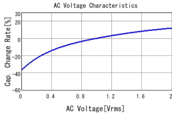
■ GRM188R71C105ME15 C-AC Voltage capchange, DCOV, 25.0d
