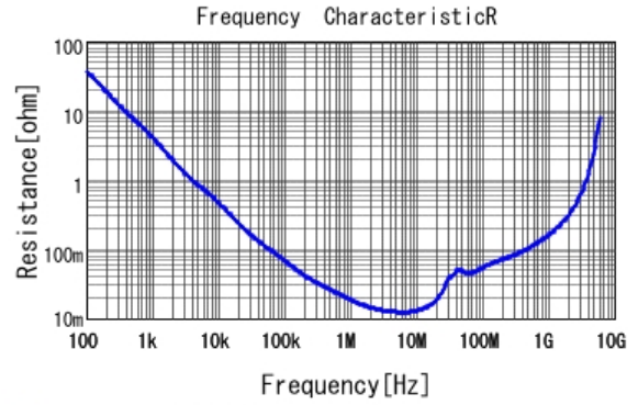
■ GRM188R71C224KA01 R DCOV, 25degC
