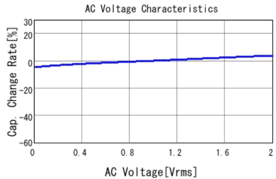
■ GRM188R71C224KA01 C-AC Voltage capchange, DCOV, 25.0d
