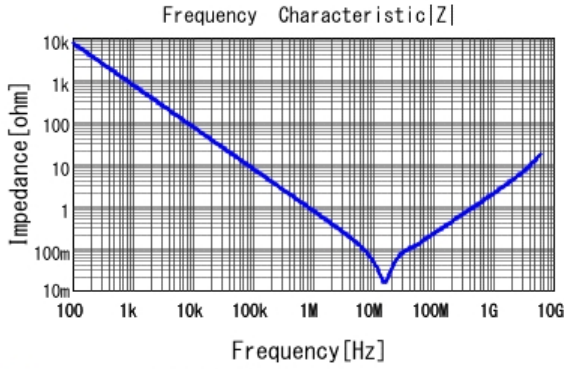
■ GRM188R71C224KA01 |Z| DCOV, 25degC
