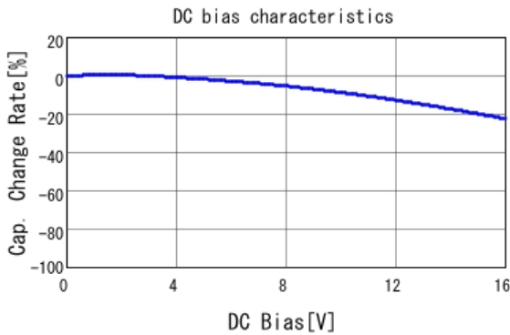
■ GRM188R71C224KA01 C-DC bias capchange, 25.0degC, AC1.
