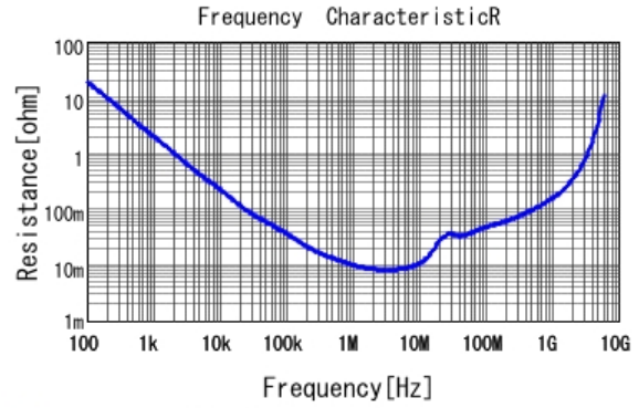
■ GRM188R71C474KA88 R DCOV, 25degC
