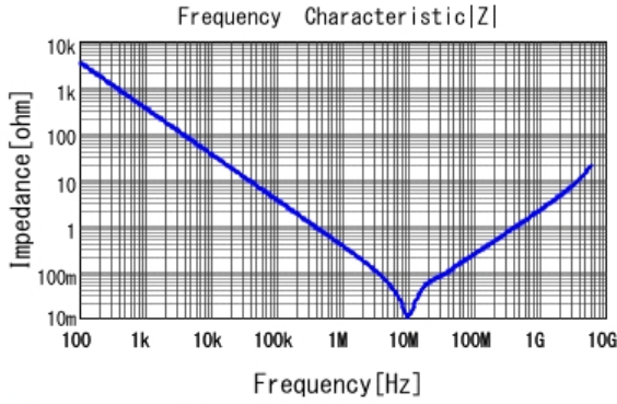
■ GRM188R71C474KA88 |Z| DCOV, 25degC
