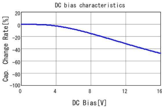
■ GRM188R71C474KA88 C-DC bias capchange, 25.0degC, AC1.
