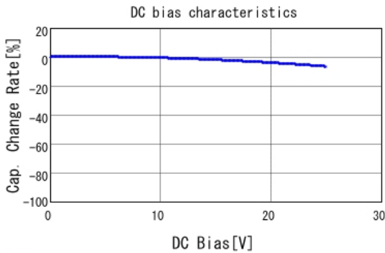
■ GRM188R71E103KA01 C-DC bias capchange, 25.0degC, AC1.
