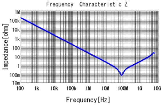
■ GRM188R71E103KA01 |Z| DCOV, 25degC
