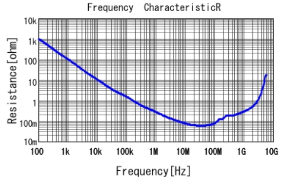
■ GRM188R71E103KA01 R DCOV, 25degC
