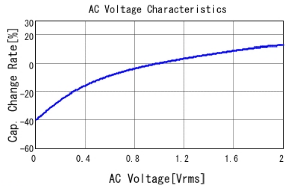
■ GRM188R71E105KA12 C-AC Voltage capchange, DCOV, 25.0d
