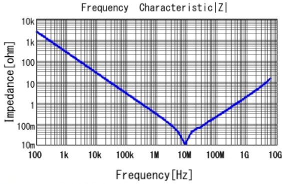
■ GRM188R71E105KA12 |Z| DCOV, 25degC
