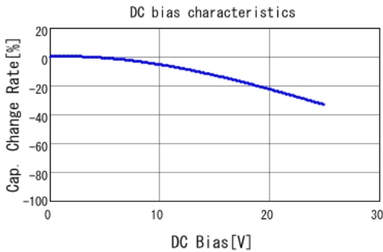
■ GRM188R71E154KA01 C-DC bias capchange, 25.0degC, AC1.
