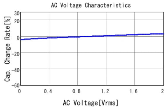
■ GRM188R71E154KA01 C-AC Voltage capchange, DCOV, 25.0d
