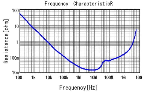
■ GRM188R71E154KA01 R DCOV, 25degC
