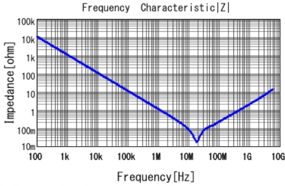
■ GRM188R71E154KA01 |Z| DCOV, 25degC
