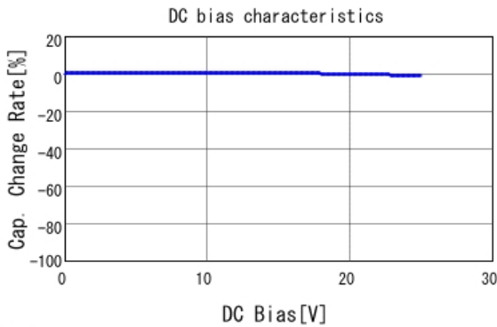
■ GRM188R71E272KA01 C-DC bias capchange, 25.0degC, AC1.
