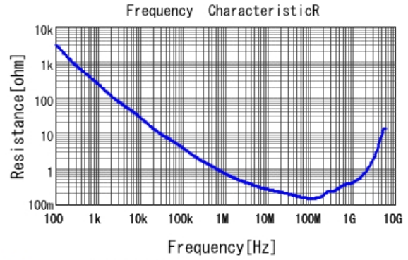
■ GRM188R71E272KA01 R DCOV, 25degC
