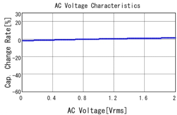
■ GRM188R71E272KA01 C-AC Voltage capchange, DCOV, 25.0d
