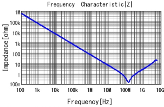
■ GRM188R71E272KA01 |Z| DCOV, 25degC
