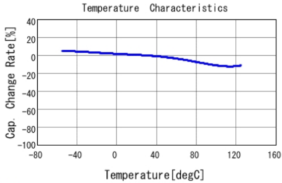
■ GRM188R71E823KA01 C-Temp. capchange, DC0.0V, AC1.0V rm
