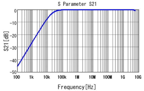
■ GRM188R71E823KA01 S21 DC0V, 25degC
