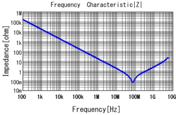
■ GRM188R71H103JA01 |Z| DCOV, 25degC
