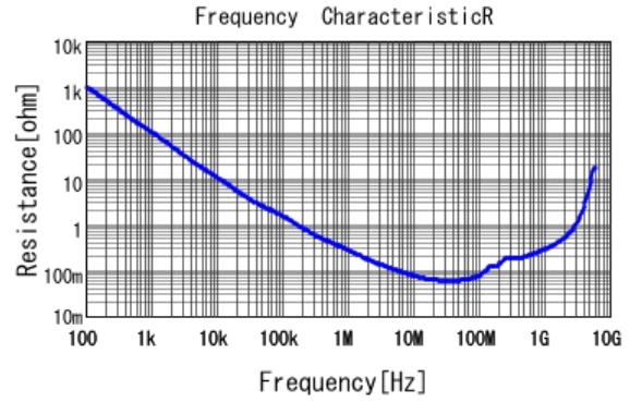
■ GRM188R71H103JA01 R DCOV, 25degC
